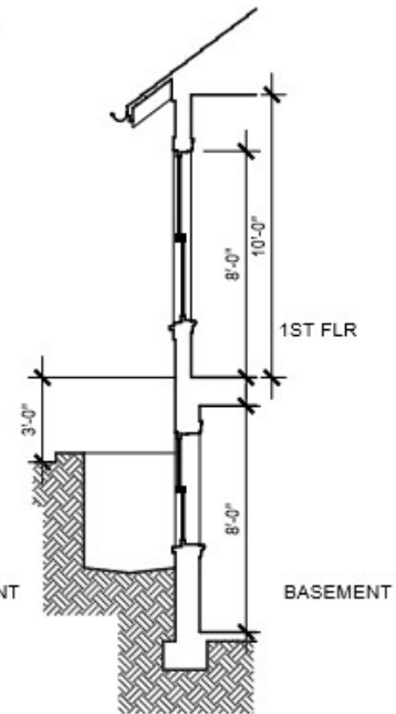
Section, 1 Story
