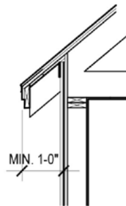
Open Eave, Exposed Shaped Rafter Tails
